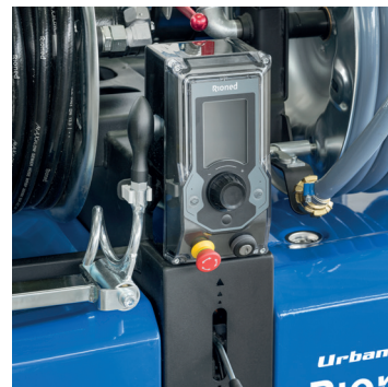
eControl+ with LCD display interface
